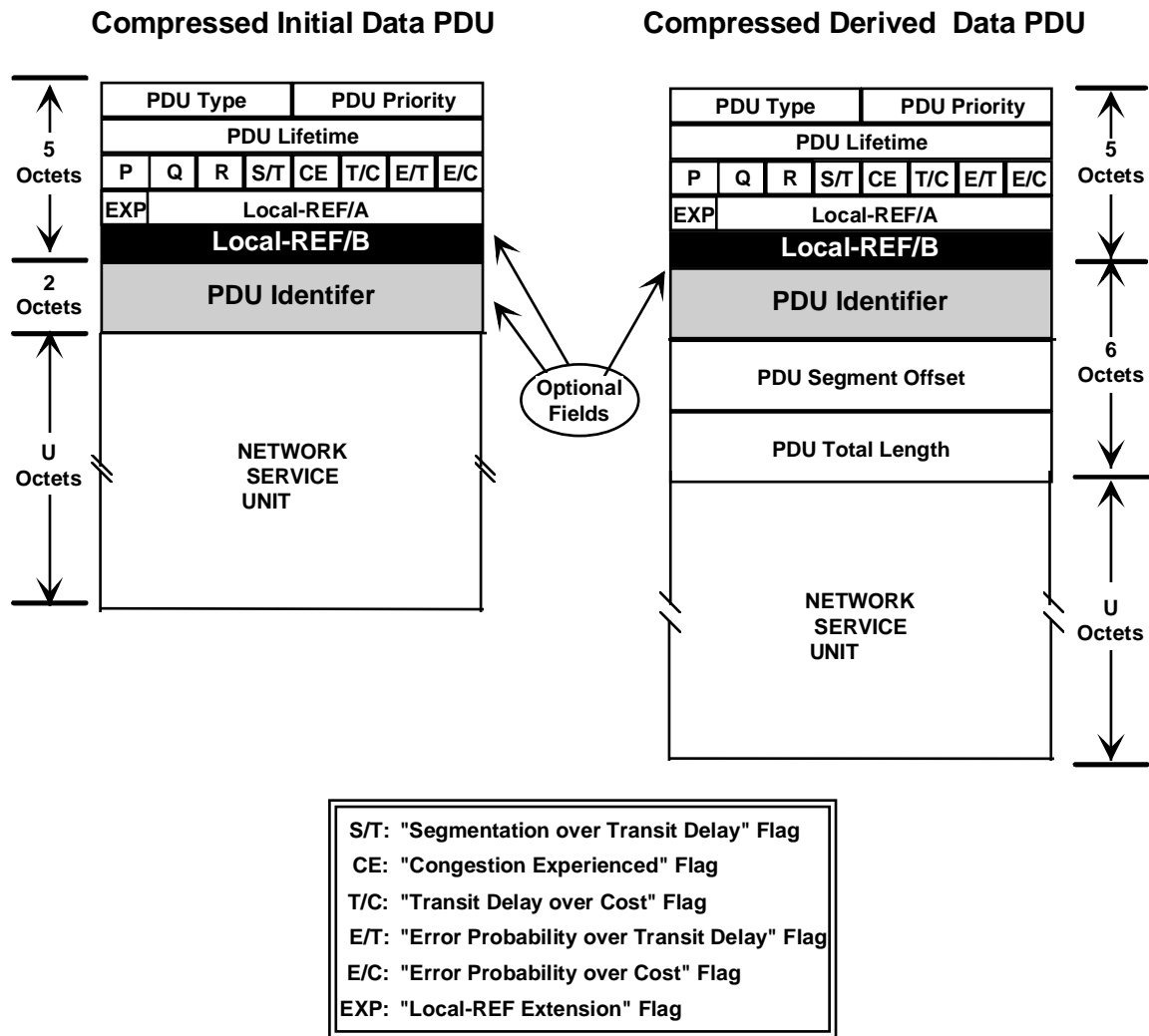
Figure 5.5.77-54 Compressed Initial and Derived PDU Formats
