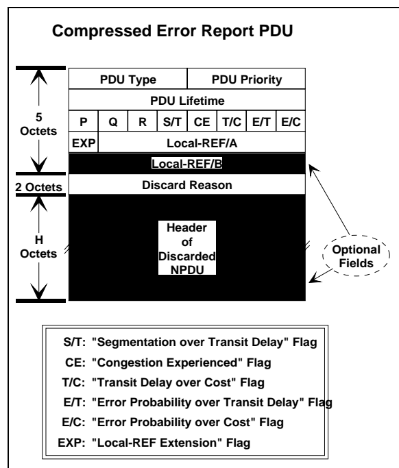
Figure 5.5.77-65 Compressed Error Report PDU
