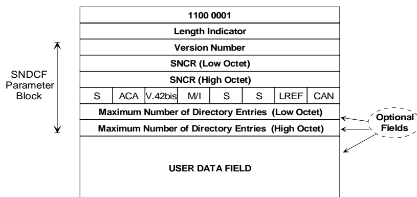
Figure 5.5.77-2 Format for Call Request User Data
